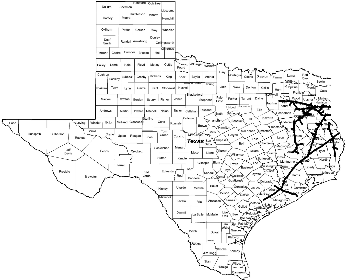
Pipeline Diameter: 2" – 42"
